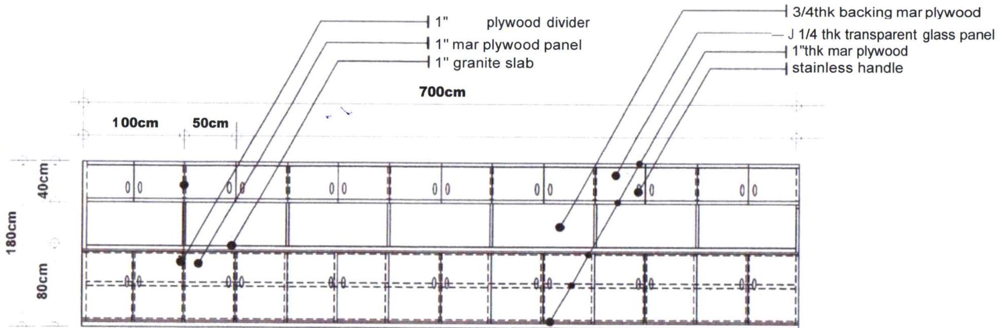
FRONT VIEW
